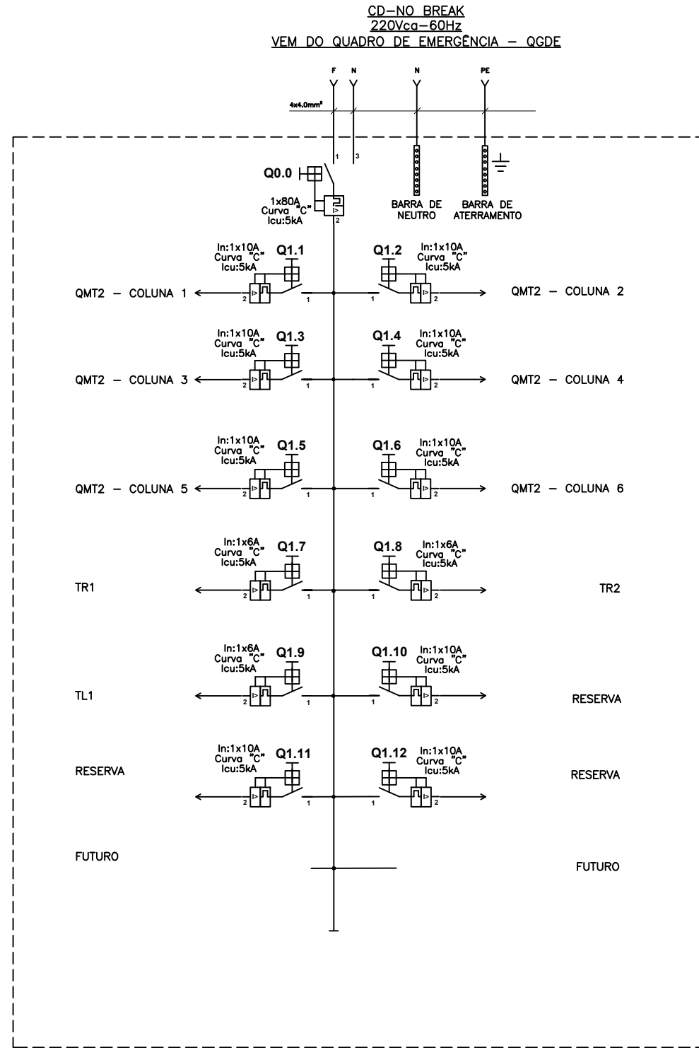
DIAGRAMA TRIFILAR CD NO-BREAK
